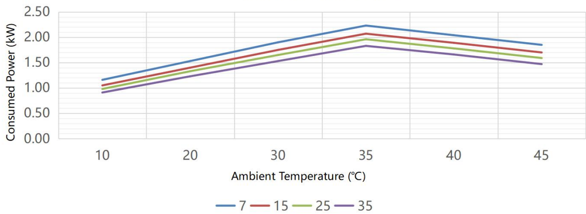
Consumed Power Curve
