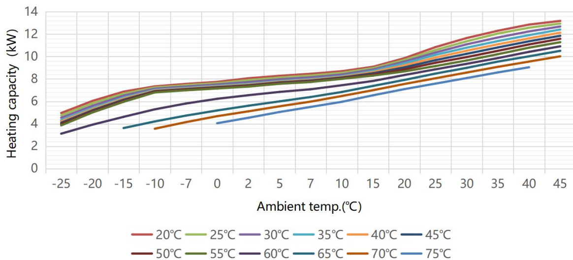
Heating Capacity Curve
