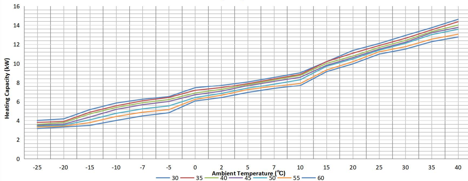
Capacity Curve
